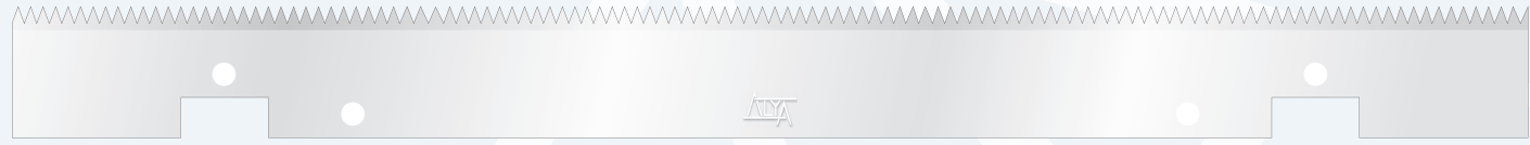
Dişli Bıçak/Toothform Knife 405x40x1mm, Tek Taraftan/Single Side 3.5 mm Diş/Tooth, 2x7mm Delik/Hole, 2xAçık Yuva/Slot, 420 Paslanmaz/Stainless
