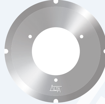
Dairesel Bıçak/Circular Knife 81.25x32x1mm, Çift Bileme/Double Bevel, 3x4.3mm Delik/Hole, 4xPerfore/Perforated, 420 Paslanmaz/Stainless
